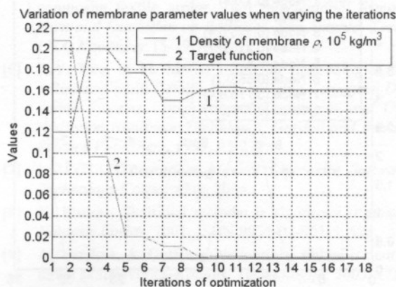
Figure 10. The variation of the value optimization parameter during iterations
