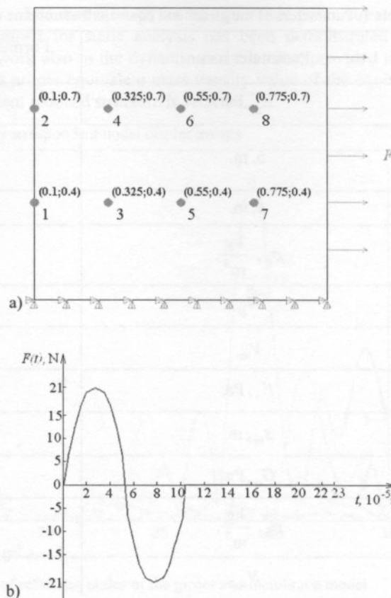
Figure 9. a) The reference nodes of the model, b) The time law of the loading force
